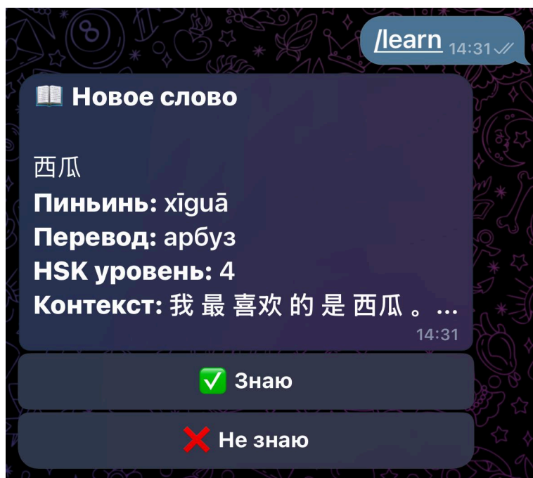
Figure 3. Flashcard displayed by /learn. The user can mark the word as known or unknown.
